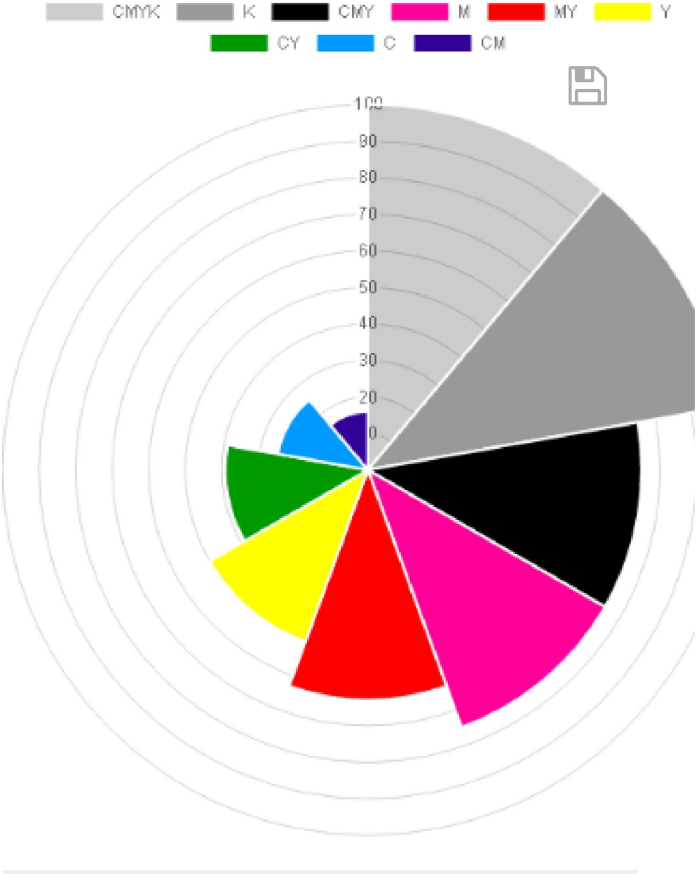
Polar Chart
