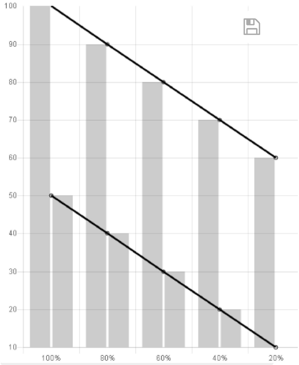
Mixed Chart
