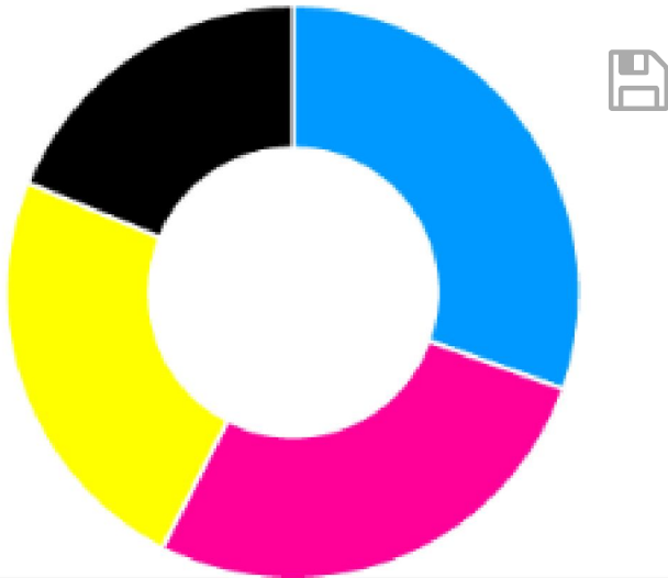
Doughnut Chart
