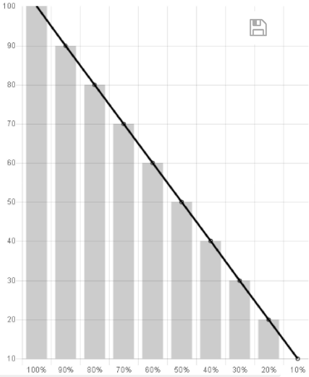
Line Chart
