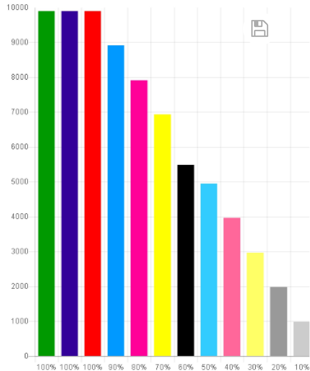
Bar Chart
