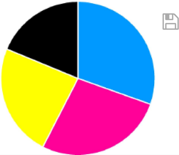
Pie Chart
